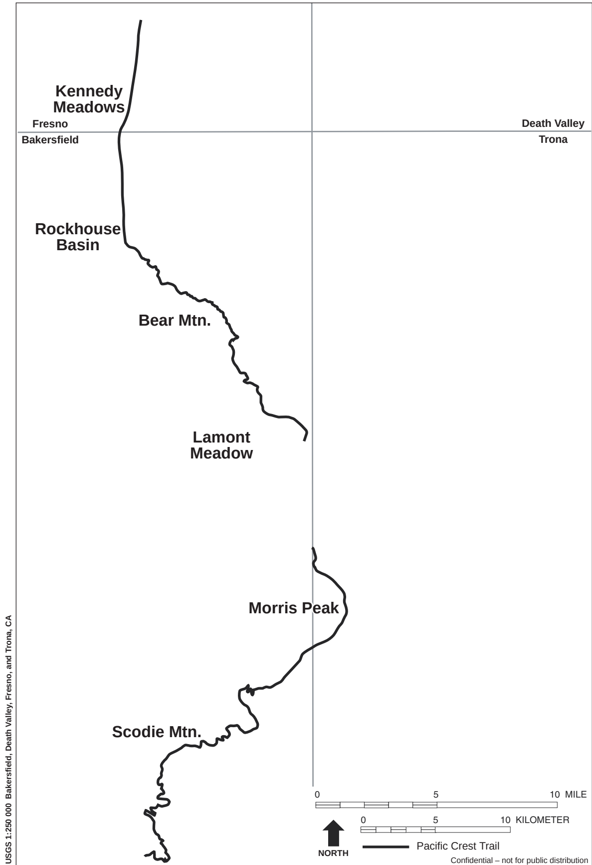
Figure 1.3 Map of the Pacific Crest Trail Segments and Study Area.
