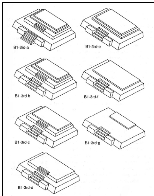
Figure 5. Reconstruction of Blackman Eddy Structures B1-3 rd -g through B1-3 rd -a (from Garber 2004a:43).
